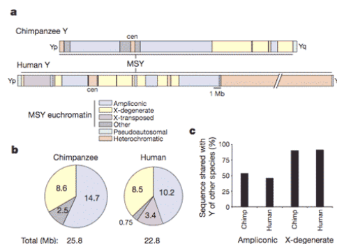
Figure 1 | Comparison of chimpanzee and human Y chromosomes. a , Schematic representations of chromosomes. cen, centromere; Yp, short arm; Yq, long arm. For both chromosomes, the MSY is indicated. Six sequence classes are shown, four of which are MSY euchromatin. ('Other' denotes MSY single-copy sequences that are not X-degenerate or X-transposed.) Chromosomes are drawn to scale, with the exception of the large heterochromatic block on human Yq. b , Sizes (in Mb) of four MSY euchromatin sequence classes in chimpanzee and human. c , Percentages of ampliconic and X-degenerate sequences present on chimpanzee Y chromosome that are also present on human Y chromosome, and vice versa.
